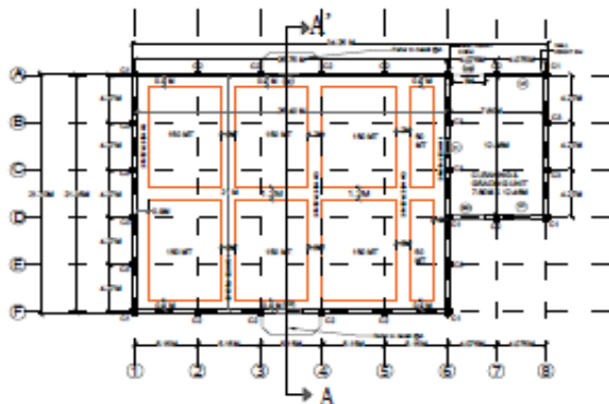
PLAN WITH STACKLINE
