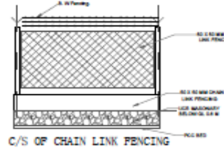
C/S OF CHAIN LINK FENCING
